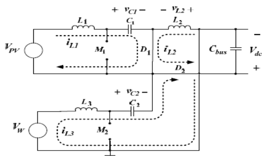
Fig 6.6: switching state (M1 off, M2 off)
