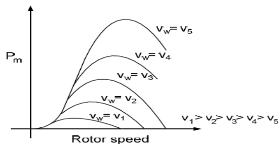
Fig 7.2: Power Curves for a typical wind turbine
