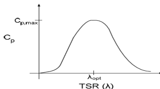
Fig 7.1: Power Coefficient Curve for a Typical Wind Turbine
