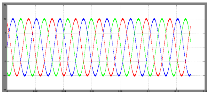
Fig 8.13: Individual Operation with only Wind source of three phase generator current
