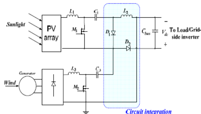
Fig 2: Both PV and wind sources are operational (CUK-SEPIC)
