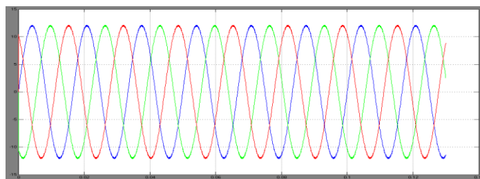
Fig 8.8: The Injected Three Phase Generator Current
