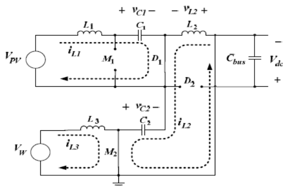
Fig 6.4: switching state (M1 off, M2 on)
