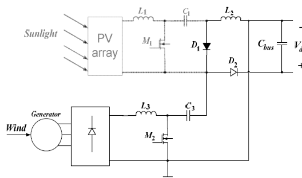
Fig 6.3: Only wind source is operational (SEPIC)
