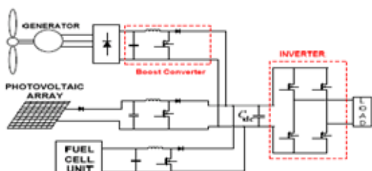
Figure 1: Hybrid system with multi-connected boost converter
