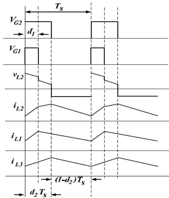
Fig 6.7: Proposed circuit inductor waveforms
