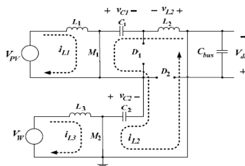
Fig 3: switching state (M1 on, M2 on)
